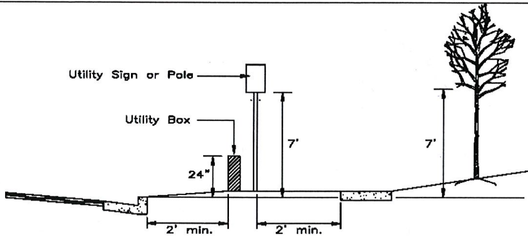
OBJECTS WITHIN SIGHT DISTANCE TRIANGLE
